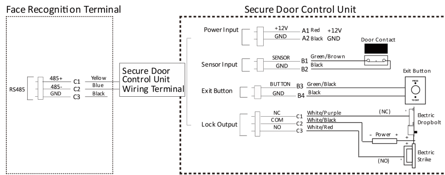
Figure 4-3 Secure Door Control Unit Wiring
