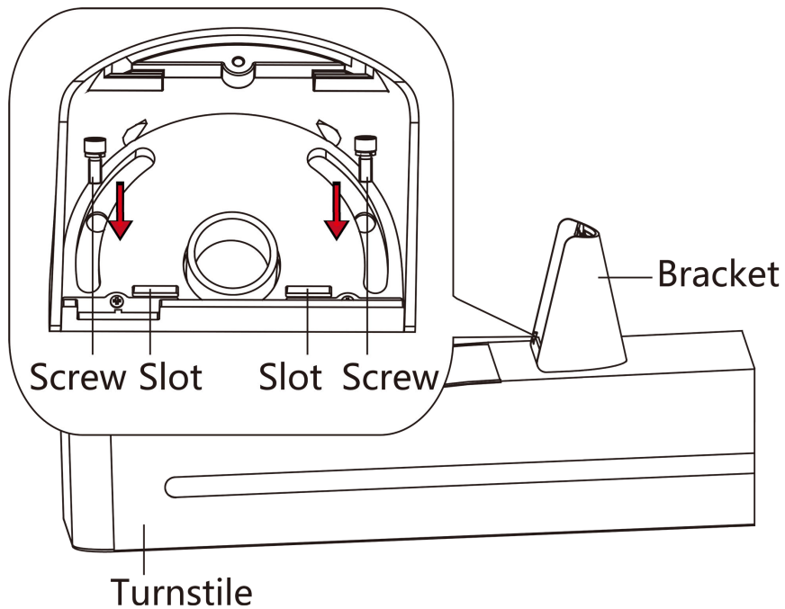
Figure 3-14 Secure Bracket
