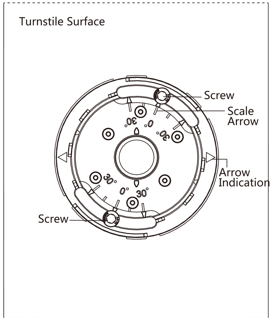
Figure 3-4 Screw Position
