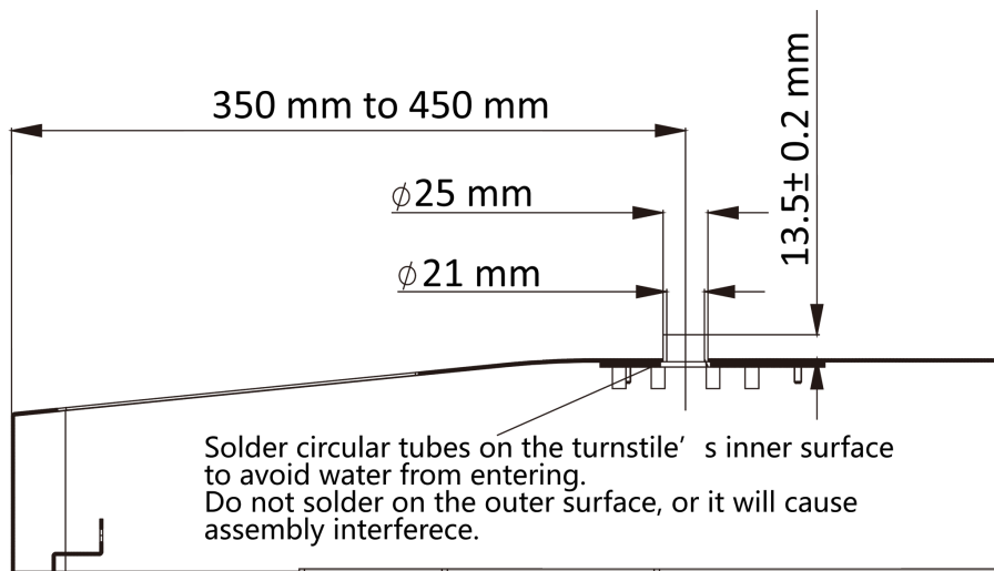
Figure 3-2 Solder Tubes
