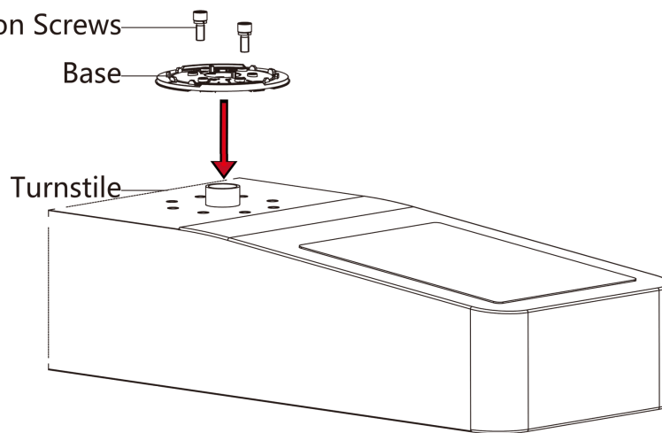
Figure 3-3 Install Base
