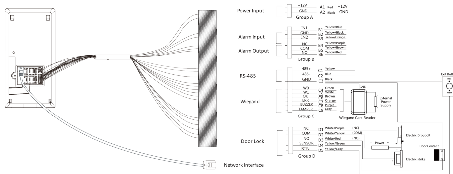
Figure 4-2 Device Wiring
