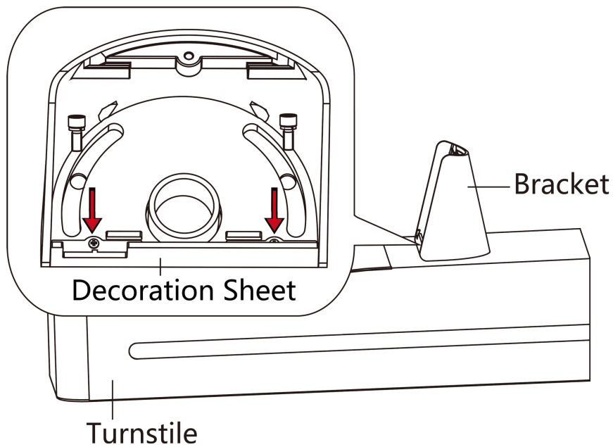
Figure 3-12 Remove Screws
