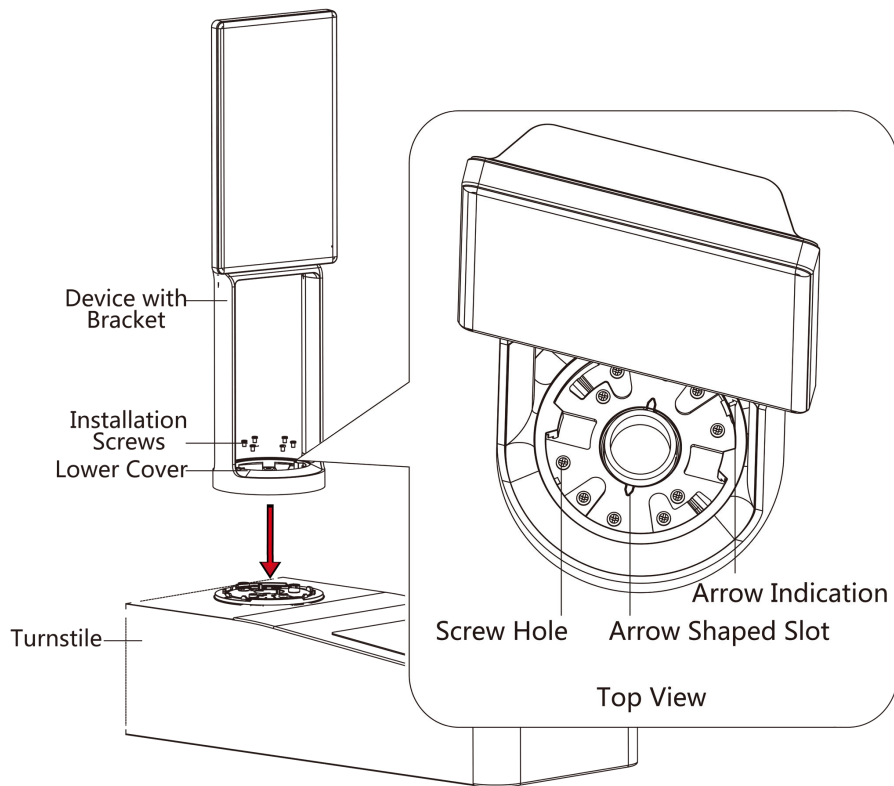
Figure 3-5 Secure Lower Cover and Turnstile
