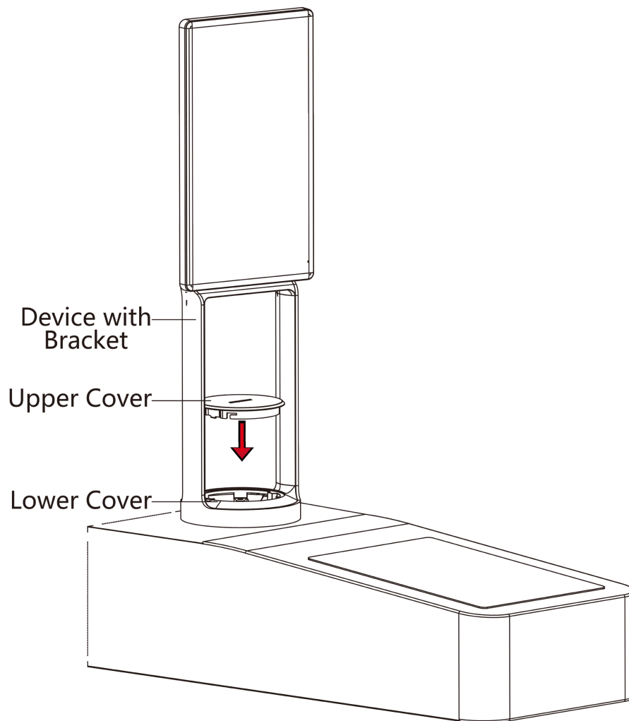
Figure 3-6 Secure Upper Cover
