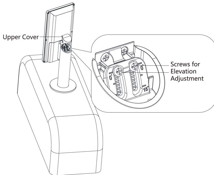
Figure 3-10 Adjust Elevation
